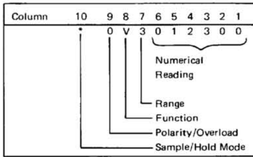
Figure 3-5. Option 021 Printout.
