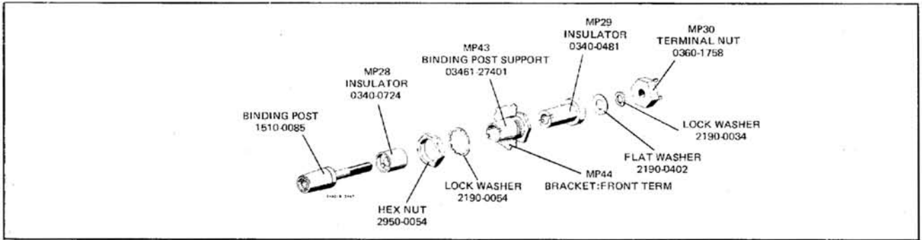
Figure 8-8. Binding Post Assembly.
