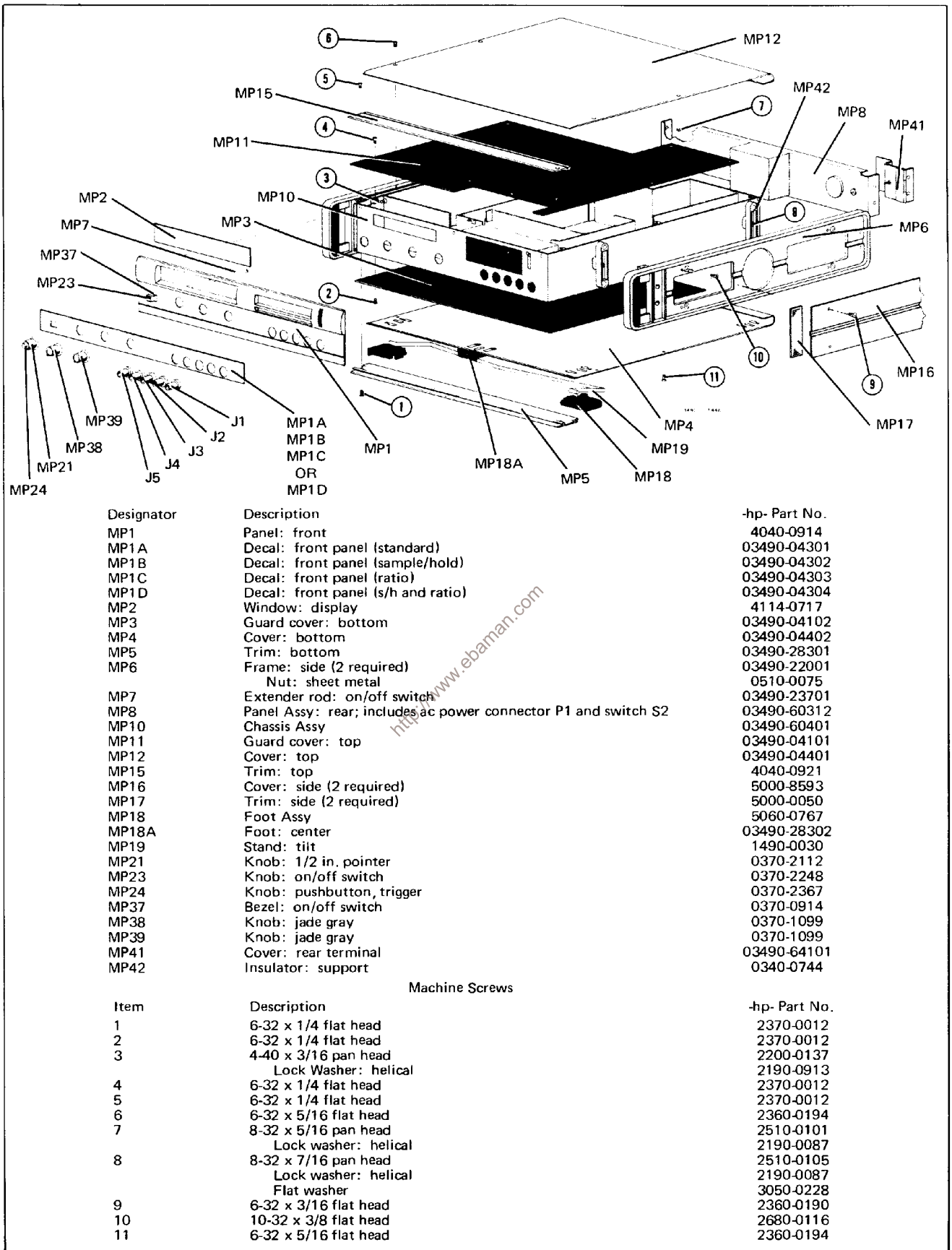
Figure 6-1. Chassis Parts.
