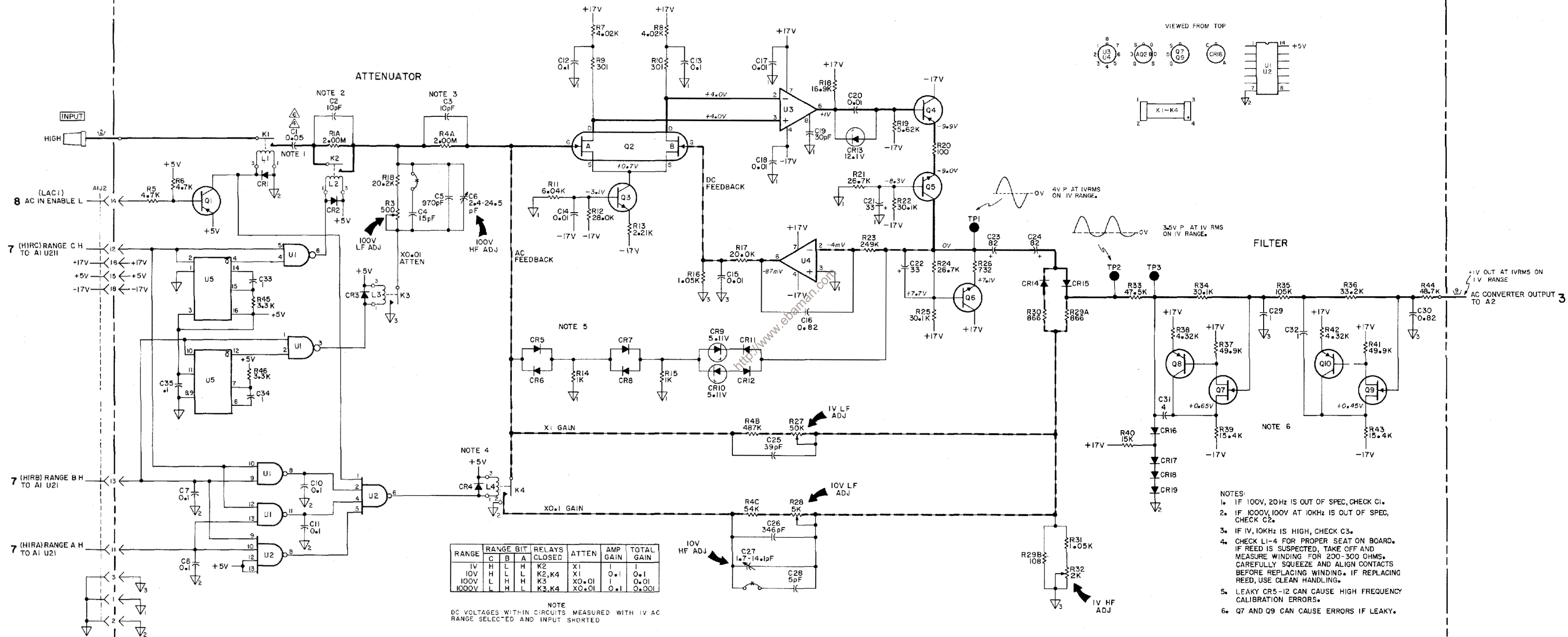
Figure 7-29. Schematic Diagram, AC Converter, A6. 7-57/7-58
