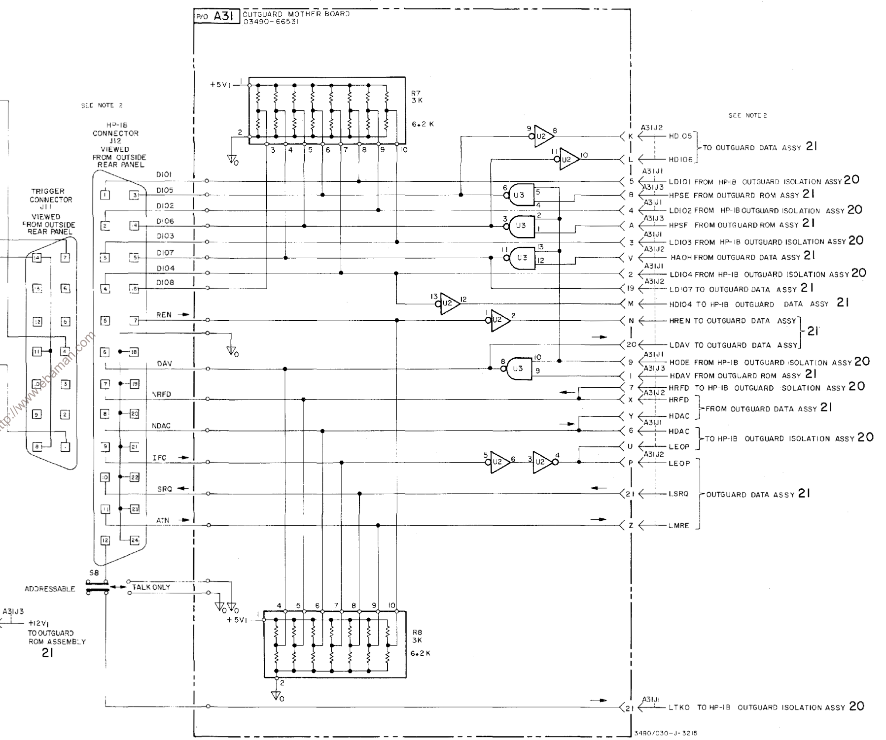
Figure 7-40. Schematic Diagram, Outguard Mother Board, A31. 7-79/7-80
