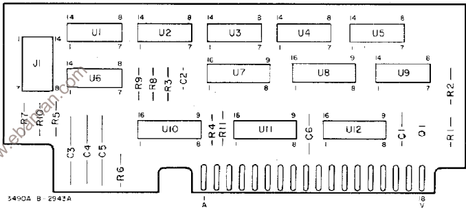
A11 hp Part No. 03490-66511 Rev. C
