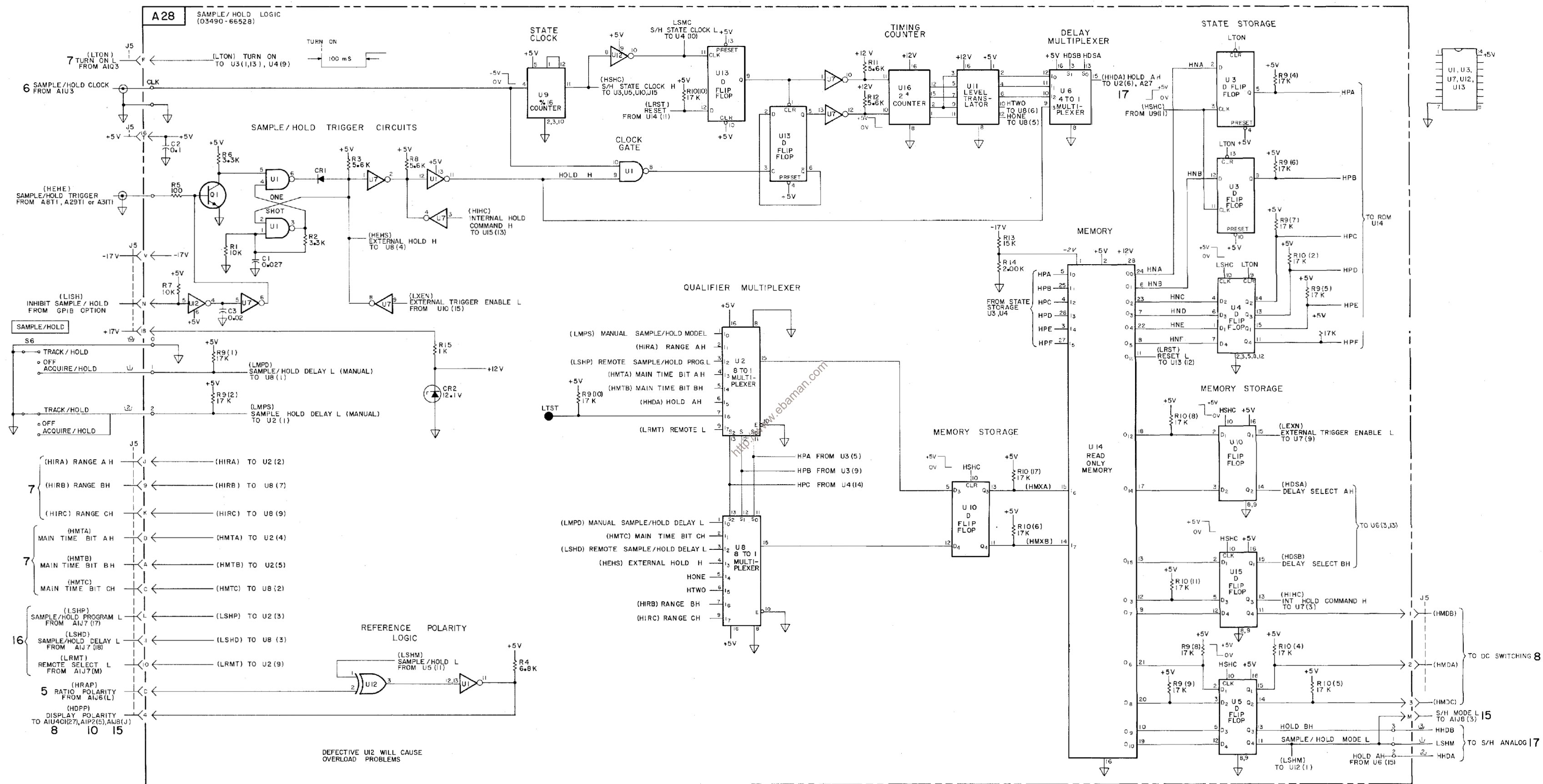
Figure 7-35. Schematic Diagram, Sample/Hold Logic Circuits, A28.
