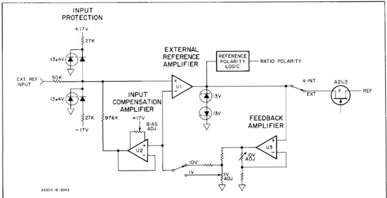
Figure 4-14. Simplified Diagram, External Reference Circuits.
