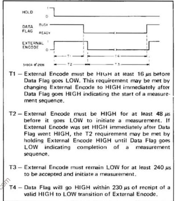
Figure 3-4. External Trigger Sequence (Option 020).
