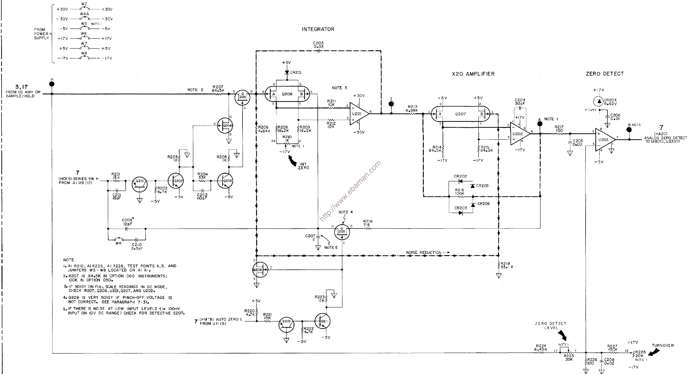
Figure 7-21. Schematic Diagram, Integrator and Zero Detect Circuits, A1.
