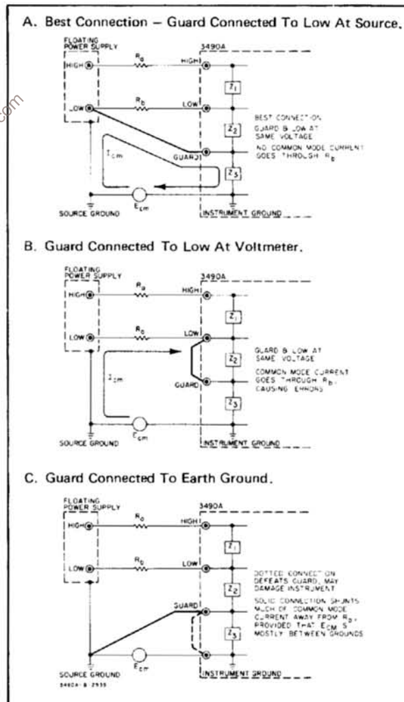
Figure 3-2. Connecting the Guard.
