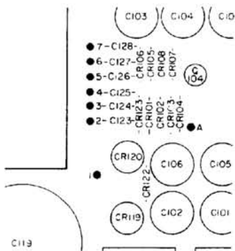
Figure 7-26. Component Locator.
