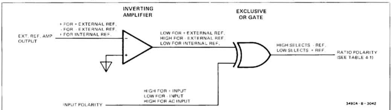
Figure 4-16. Reference Polarity Logic.
