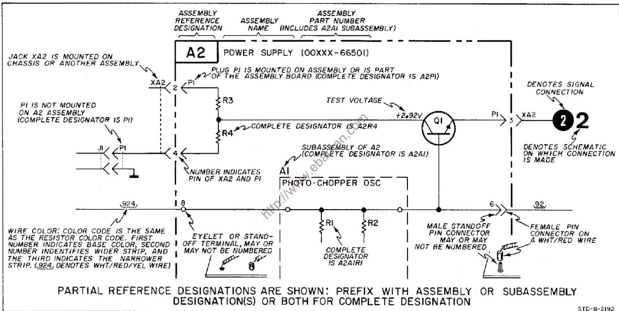
Figure 7-19. Reference Designations.
