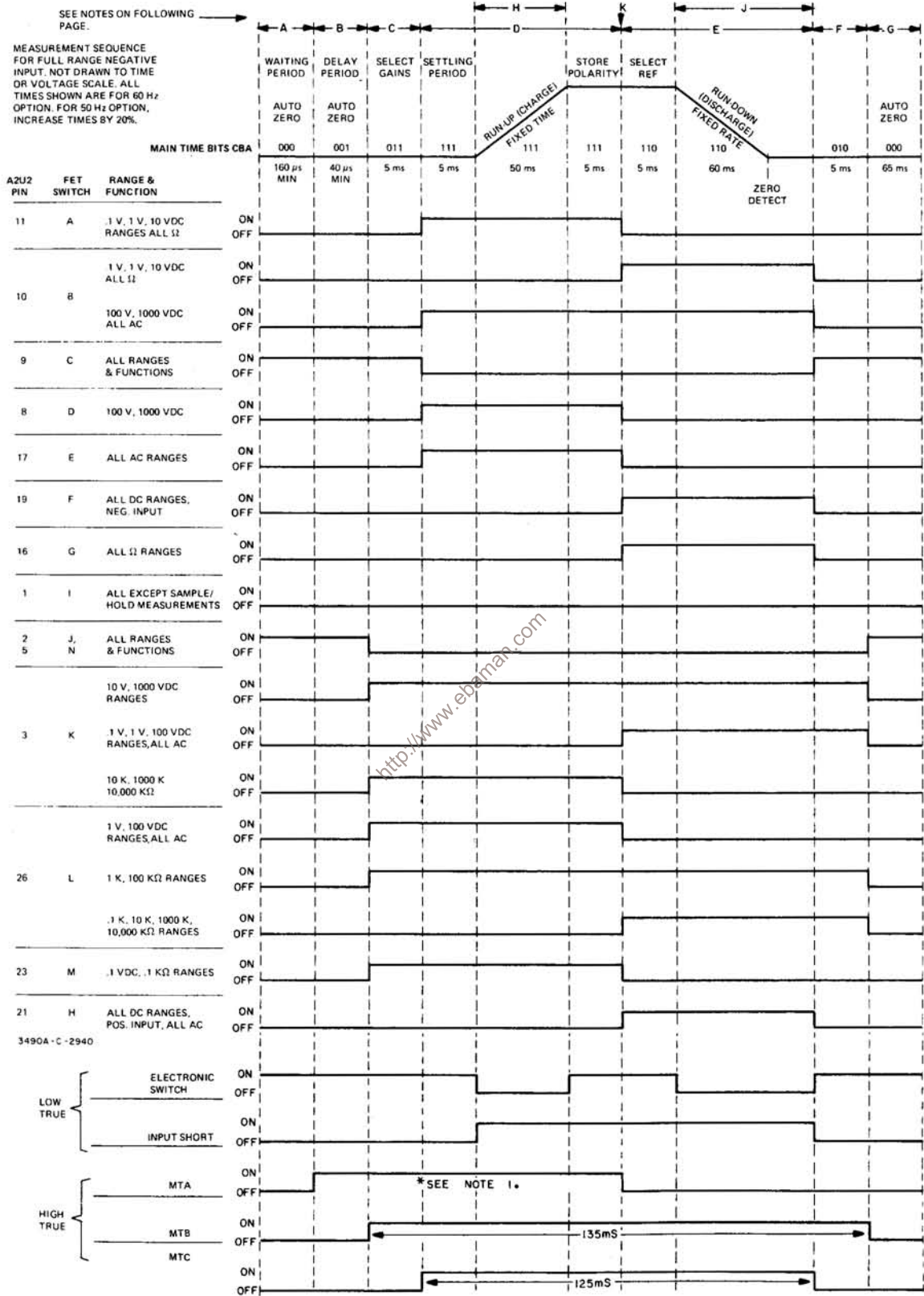
Figure 4-4(a). Measurement Sequence.
