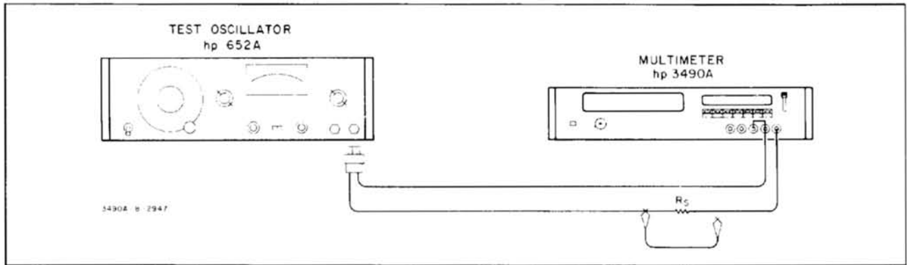
Figure 5-6. AC Voltmeter Input Impedance Test.
