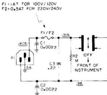
P/O Figure 7-26.
