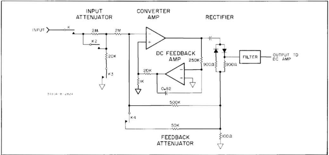
Figure 4-6. Simplified Diagram, AC Converter.
