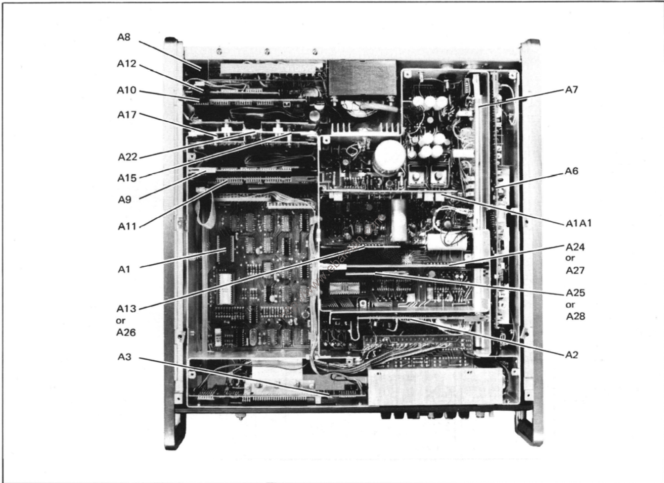
Figure 7-17. Location of Assemblies.
