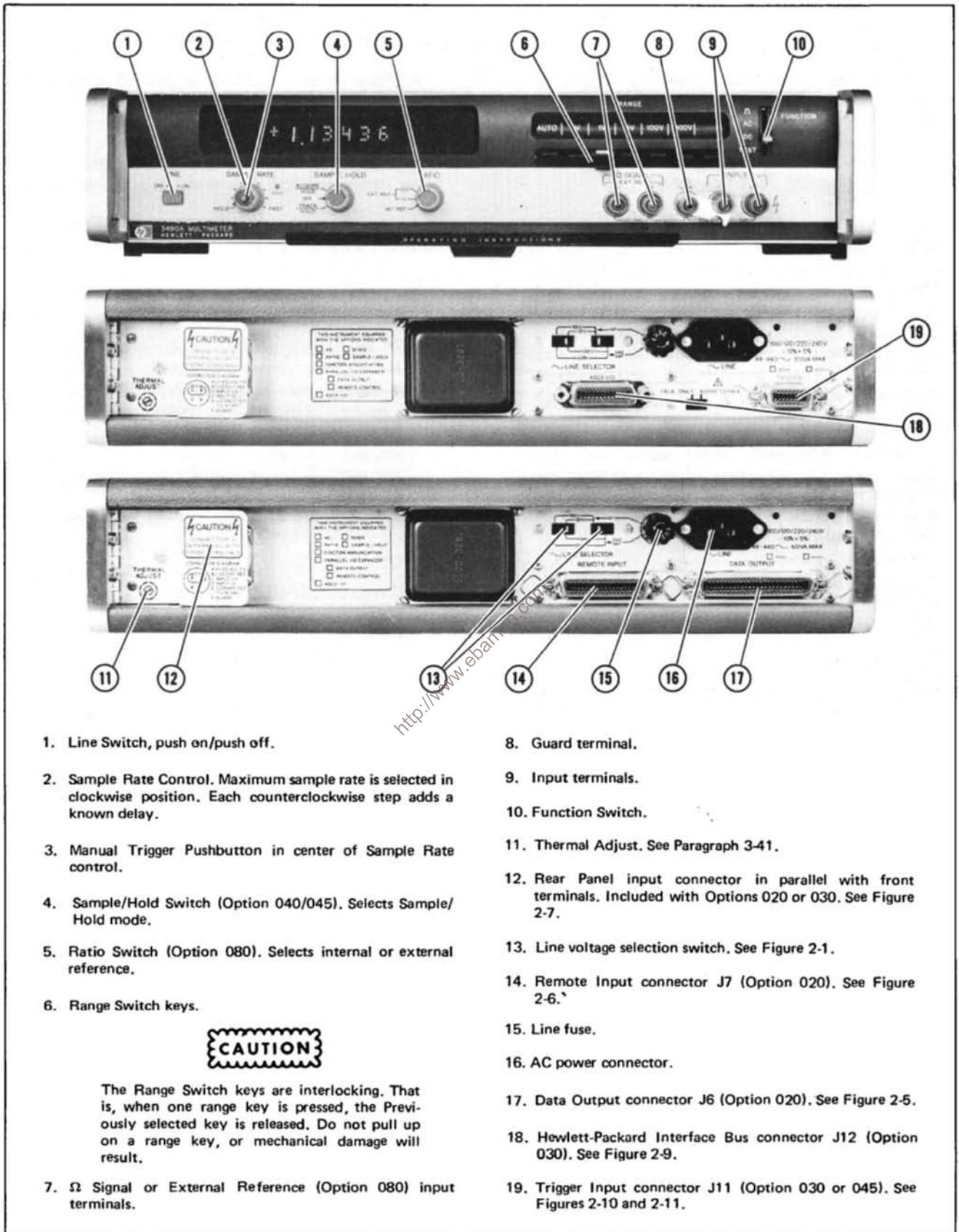
Figure 3-1. Front and Rear Panel.
