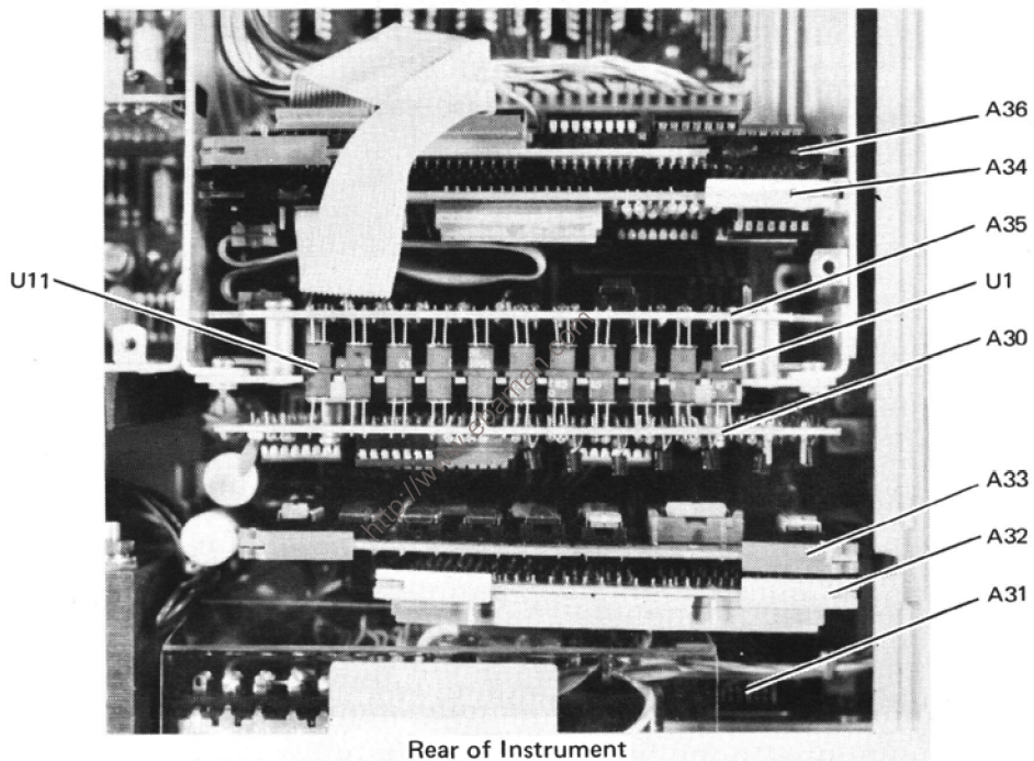
Figure 7-17. Location of Assemblies.
