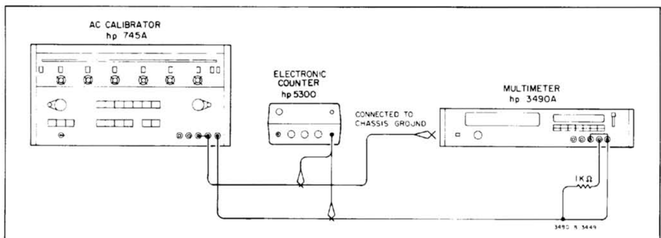
Figure 5-3. AC Common-Mode Rejection Test.
