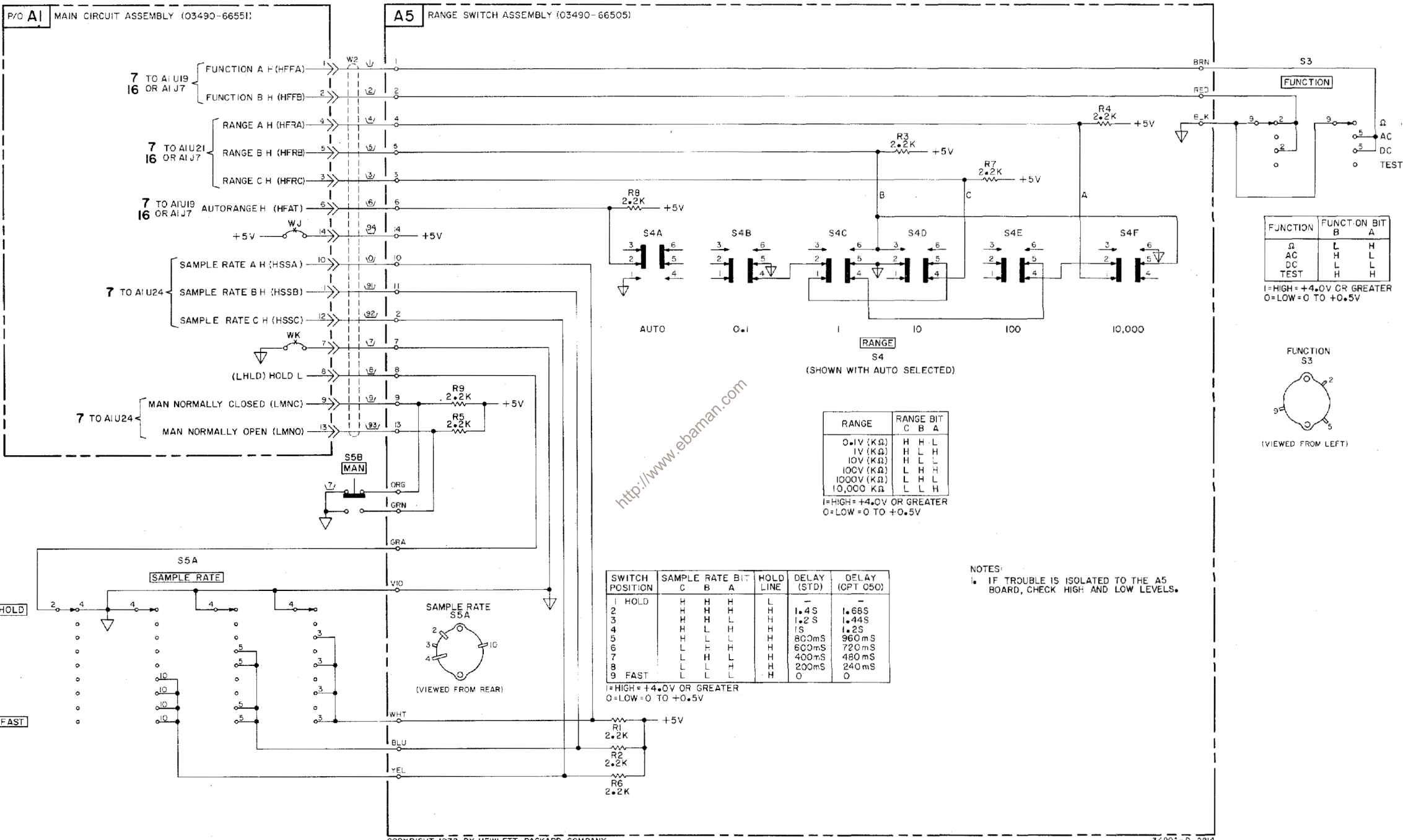
Figure 7-28. Schematic Diagram, Function, Range, and Sample Rate Switches, A5.
