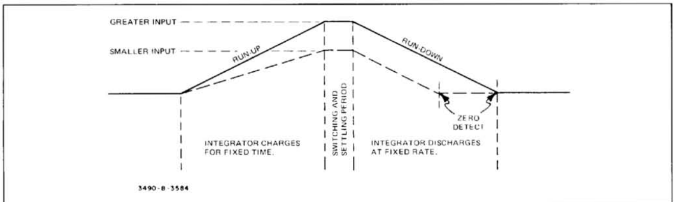
Figure 4-1. Dual-Slope Integration.
