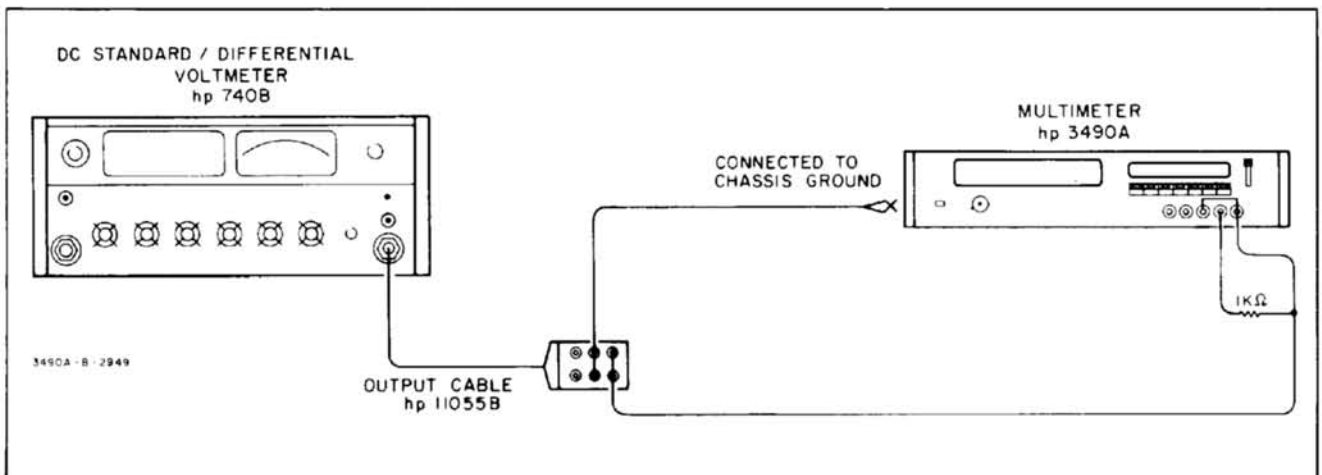
Figure 5-2. DC Common-Mode Rejection Test.
