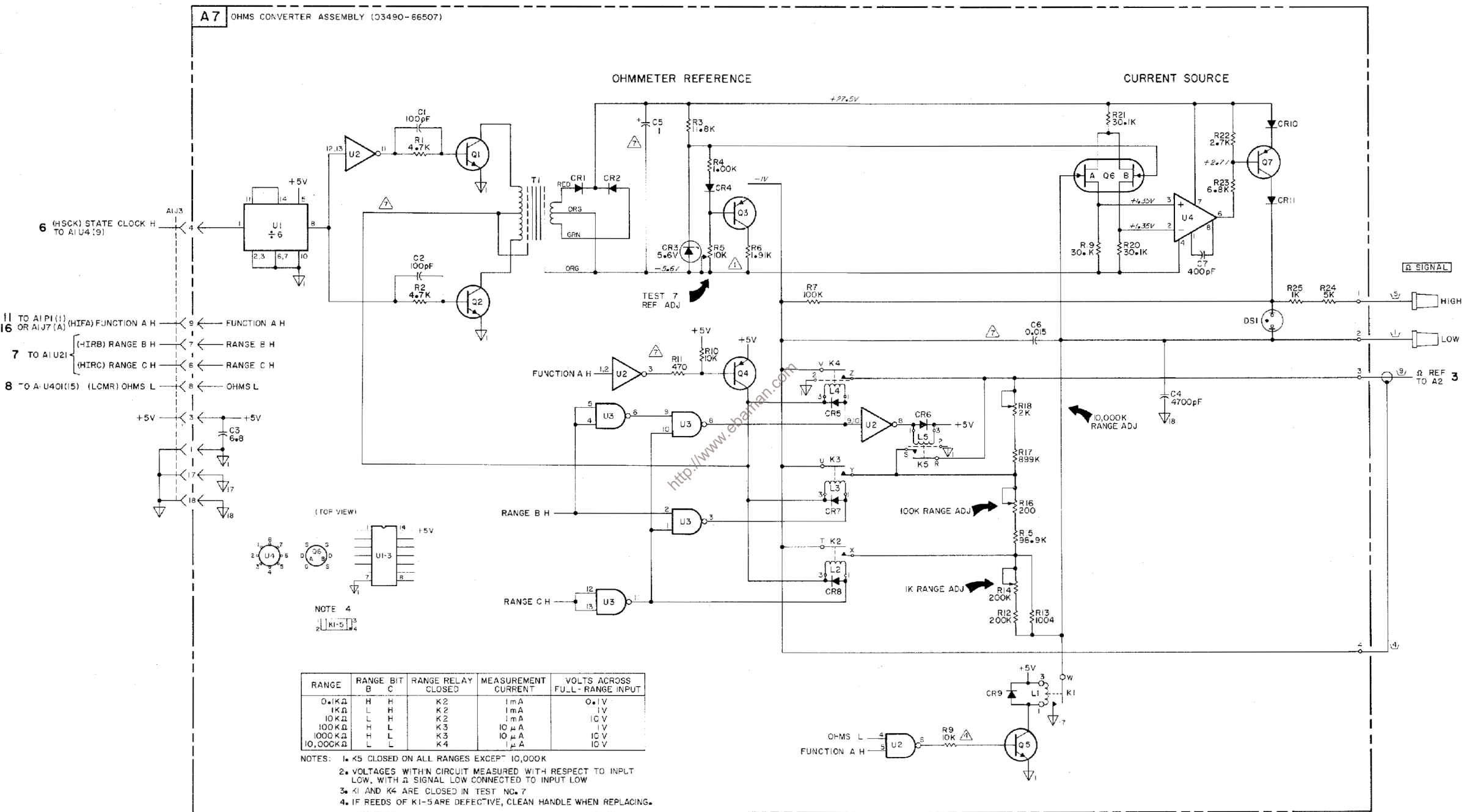
Figure 7-30. Schematic Diagram, Ohms Converter, A7. 7-59/7-60
