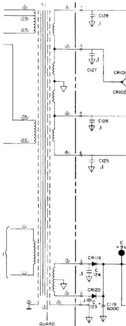
Figure 7-26. Schematic Diagram.
