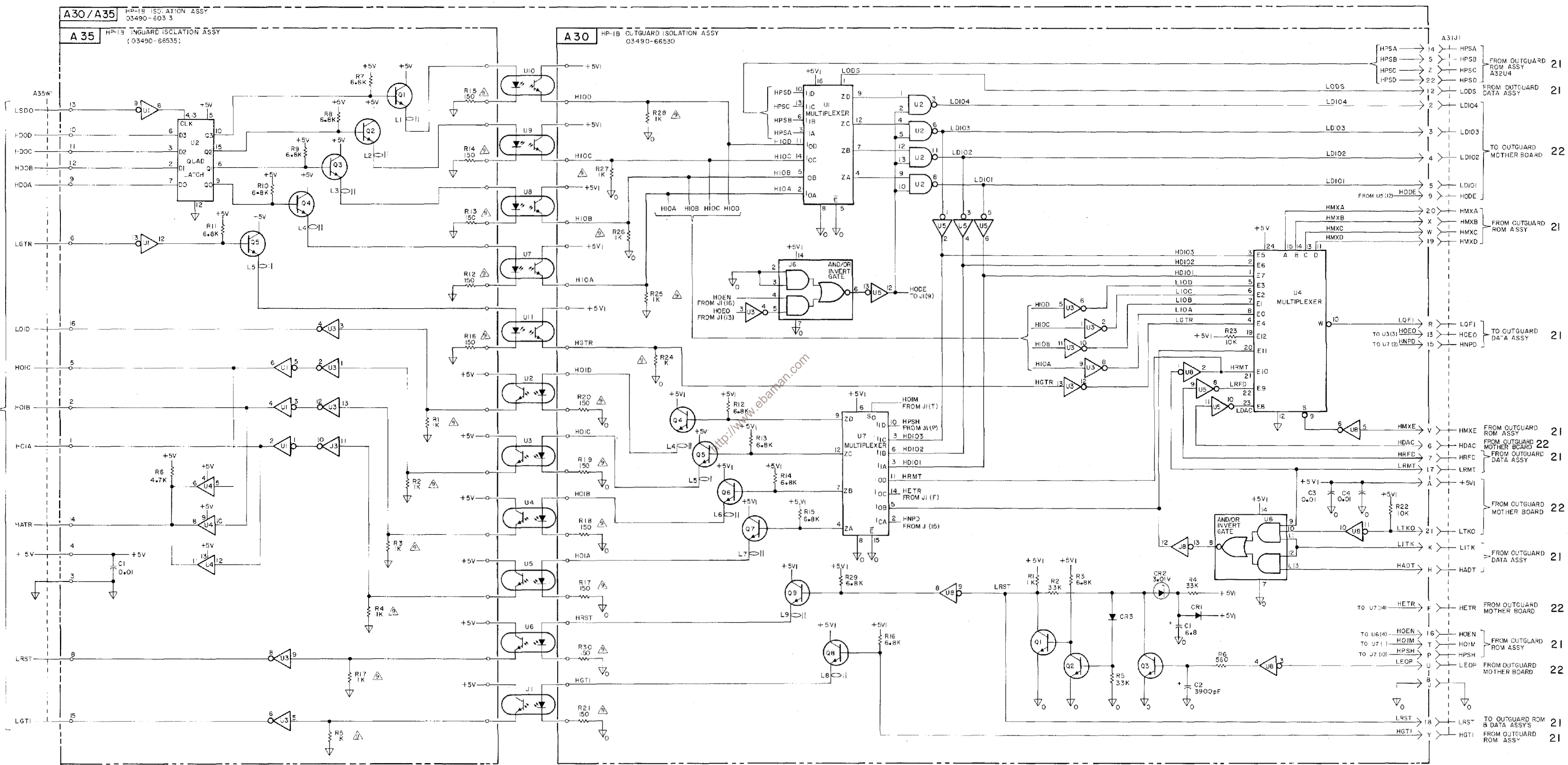
Figure 7-38. Schematic Diagram, HP-IB Isolation Assemblies, A30, A35.
