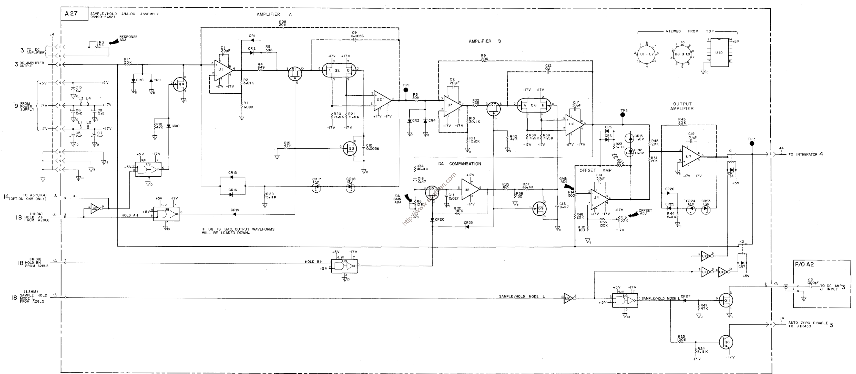
Figure 7-34. Schematic Diagram, Sample/Hold Analog Circuits, A27.
