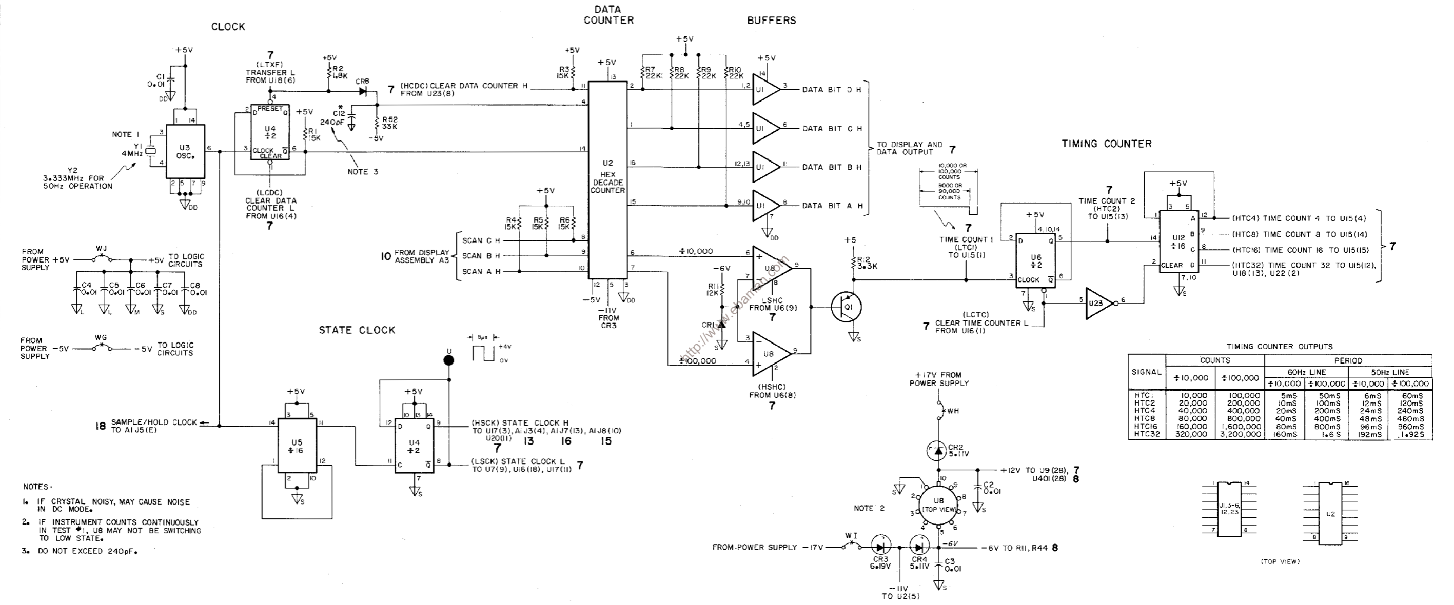
Figure 7-23. Schematic Diagram, Clock and Counters, AI.
