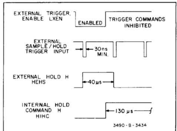
Figure 4-29. Sample/Hold Trigger Timing.
